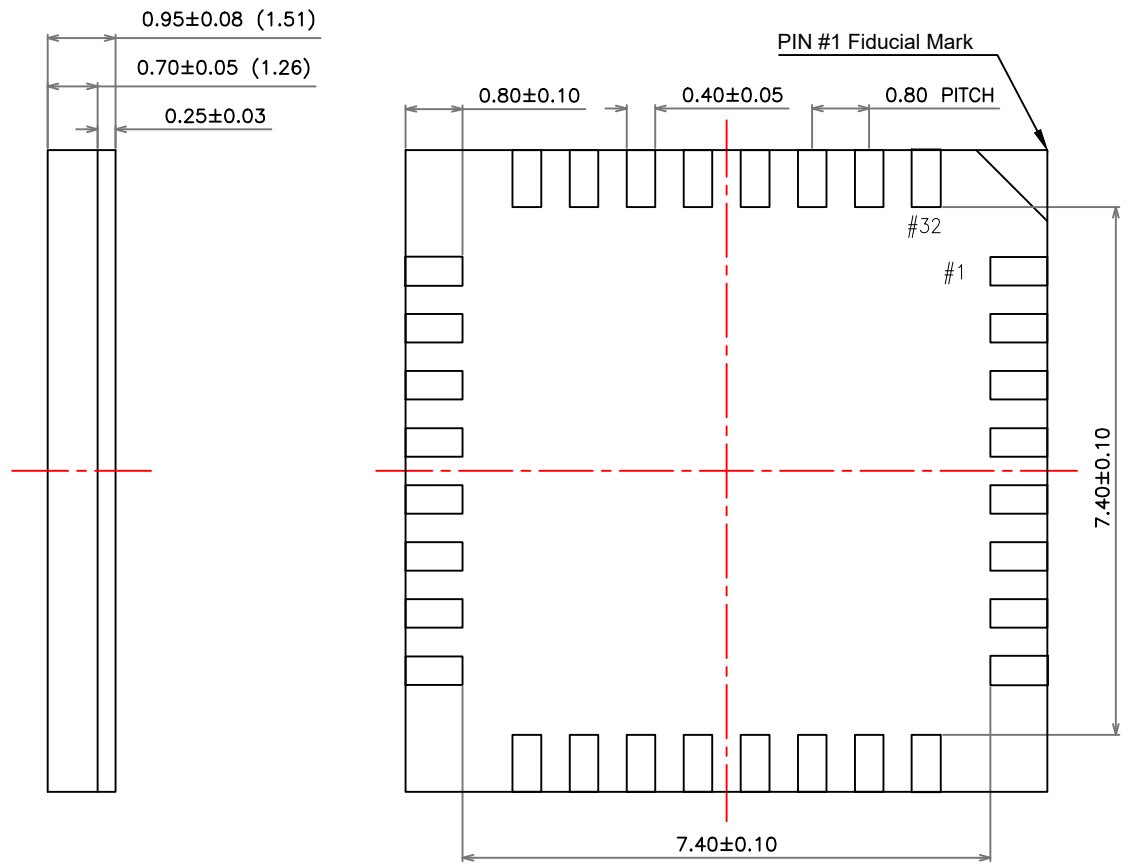
SIDE VIEW
